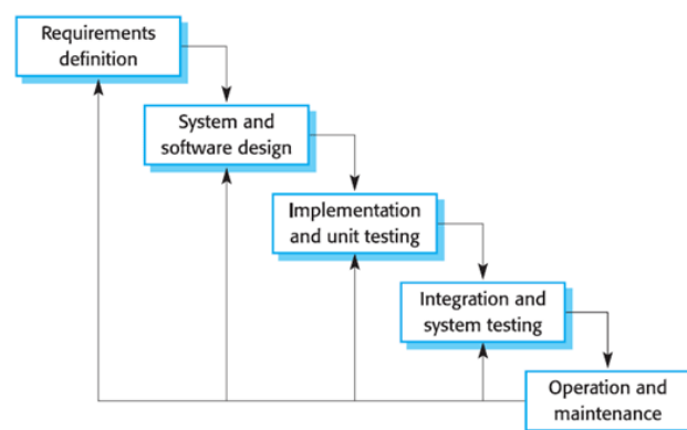
Gambar 1. Waterfall Method
