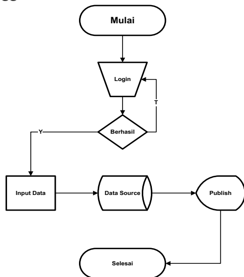
Gambar 2. Flowchart Sistem
