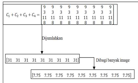
Gambar 6. Rataan FlatVector
