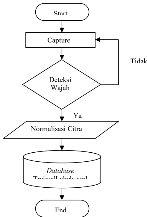
Gambar 8. Flowchart Training Wajah
