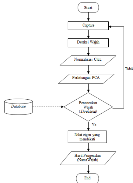
Gambar 9. Flowchart Proses Pengenalan Wajah
